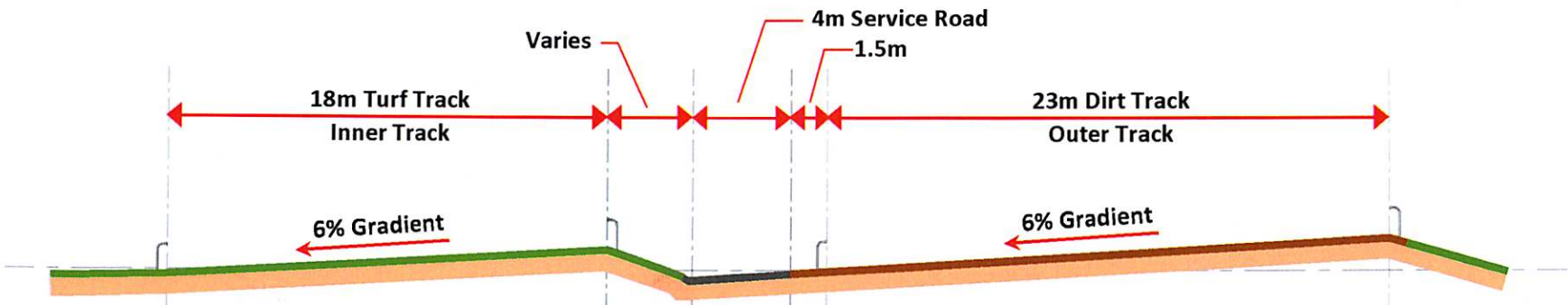
SECTION B (AT TURN)
